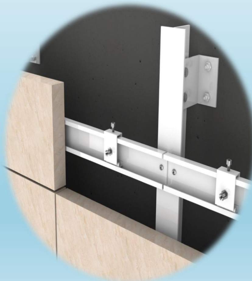
ANGLE BRACKET W/PIN
